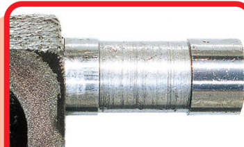
Transmission valve body spool after BG Transmission Service.
