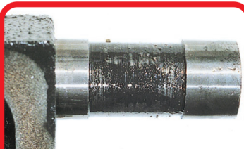
Transmission valve body spool with deposit buildup.
