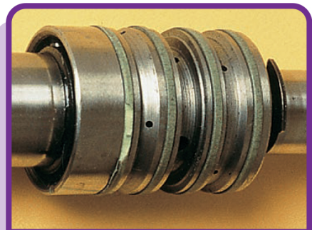
Power steering spool valve with hardened, cracked seals.
