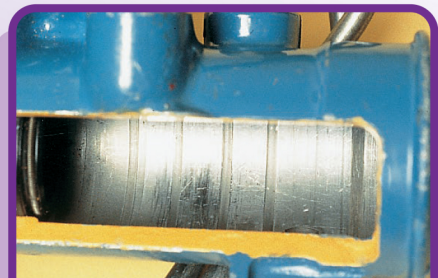
Grooves are worn into the soft metal of the spool valve housing by hardened seals.
