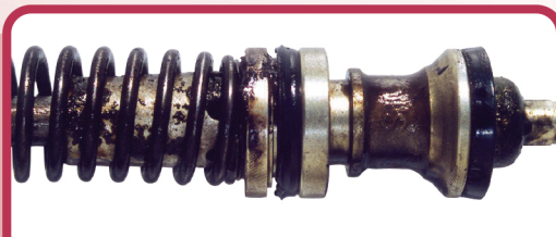
Harmful deposits and varnish buildup—resulting from worn-out, oxidized brake fluid—are apparent on this brake master cylinder piston assembly.
