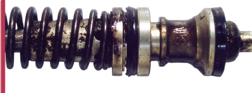
Harmful deposits and varnish buildup—resulting from worn-out, oxidized brake fluid—are apparent on this brake master cylinder piston assembly.
